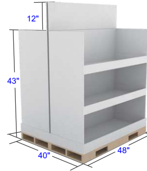
M-P007 Two-Side Floor Half Pallet Display
