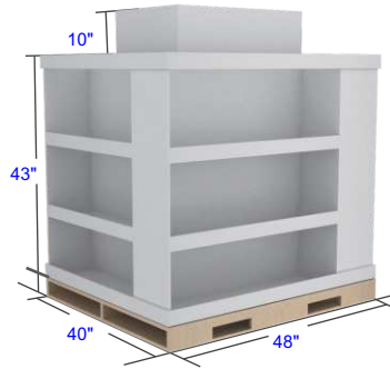
M-P011 Four Sides Full Pallet Display Shelf
