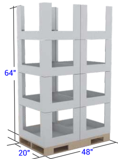
M-P004 Half Pallet
