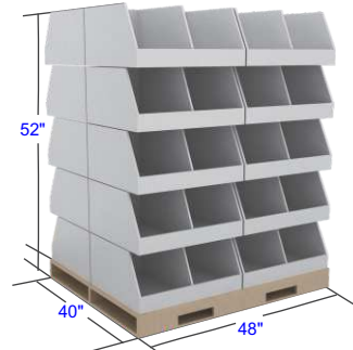
M-P005 Two Side PDQ Tray Full Pallet Display
