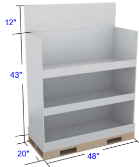
M-P007 One-Side Floor Half Pallet Display
