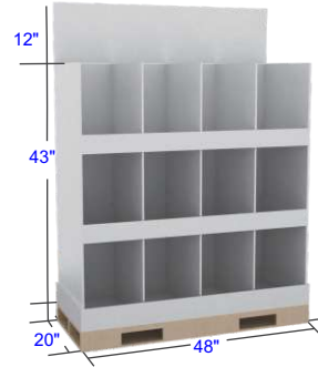
M-P007 One-Side Floor Half Pallet Display with Dividers
