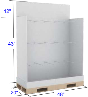
M-P009 Half Pallet Display with Hooks One-Side Floor
